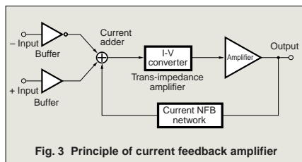
Fig. 3 Principle of current feedback amplifier
