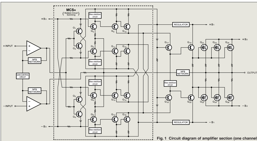
Fig. 1 Circuit diagram of amplifier section (one channel)
