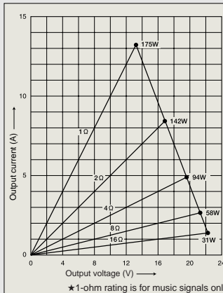
Fig. 2 Load impedance vs. output power (Output voltage/output current) ★ 1-ohm rating is for music signals only.
